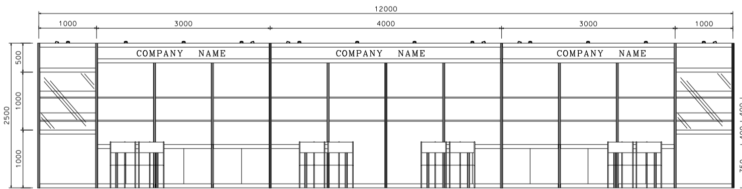
FRONT ELEVATION
