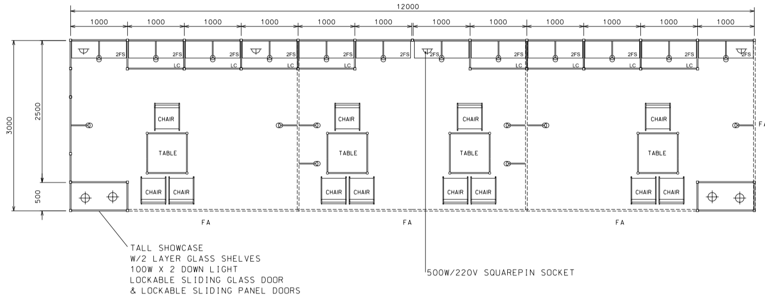
PLAN
